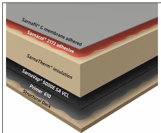
Figure 1 Typical installation
